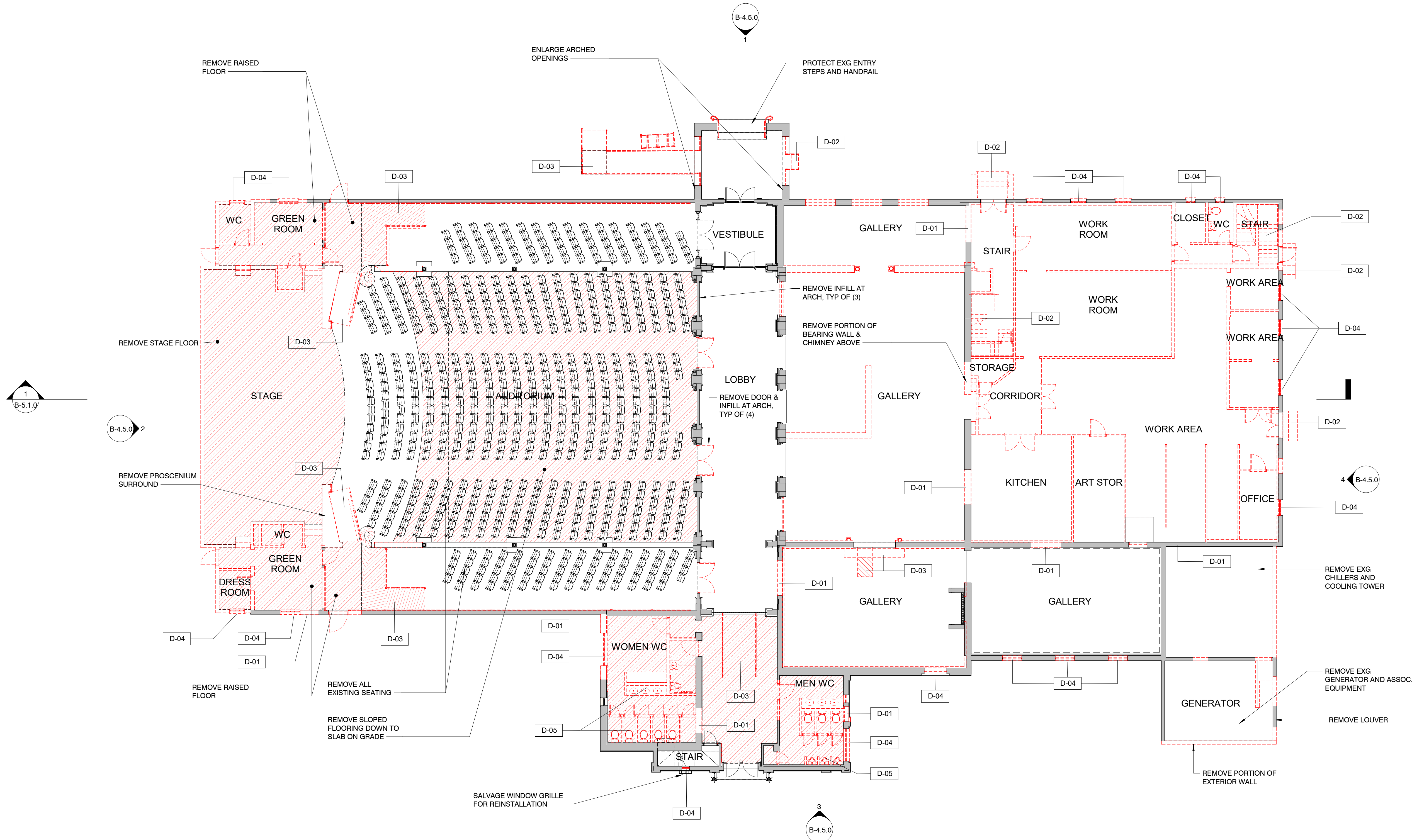
1 FIRST FLOOR MATERIAL REMOVAL PLAN B-2.1.3 3/32" = 1'-0"
