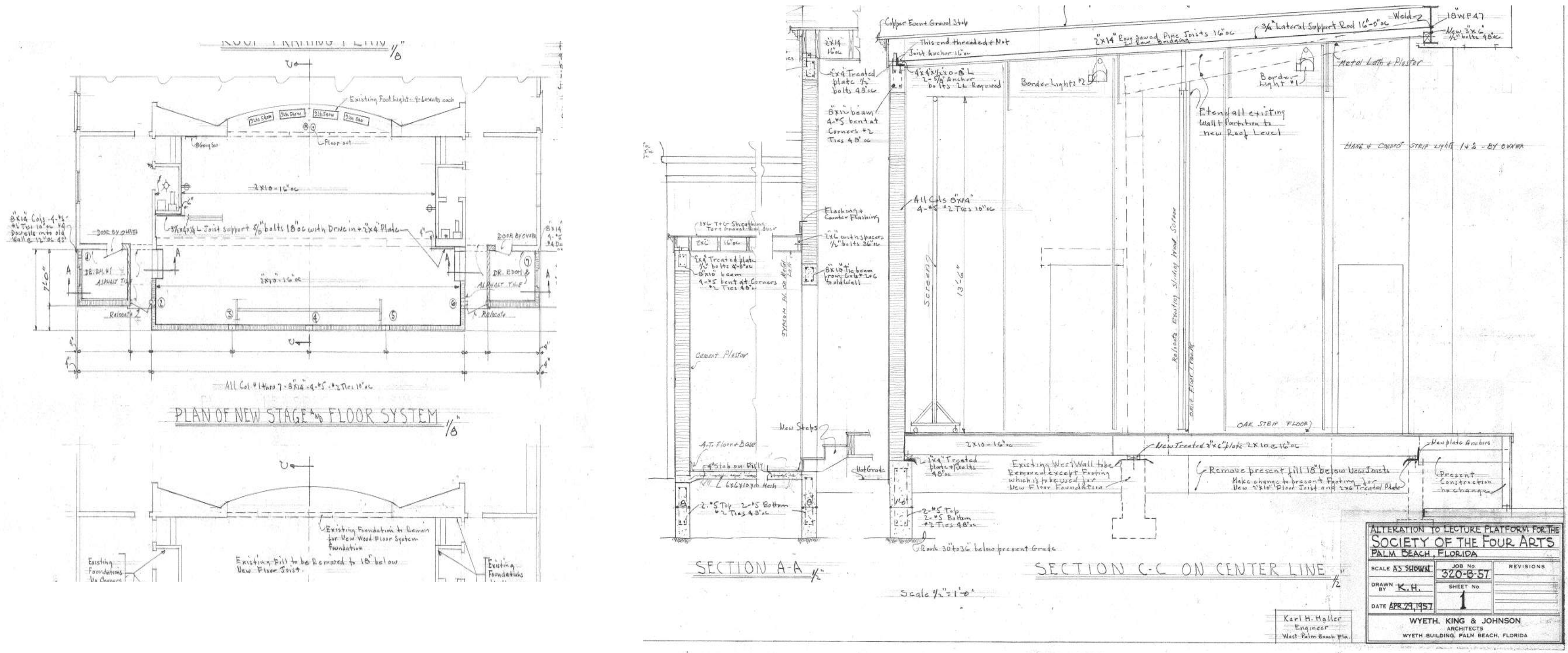
3 DETAILS FOR BACKSTAGE EXPANSION AS CONSTRUCTED - WYETH, KING & JOHNSON, 1957 B-1.0.2 SCALE IS 50% OF NOTED HISTORIC SCALE ON DRAWING - COURTESY THE PRESERVATION FOUNDATION OF PALM BEACH
