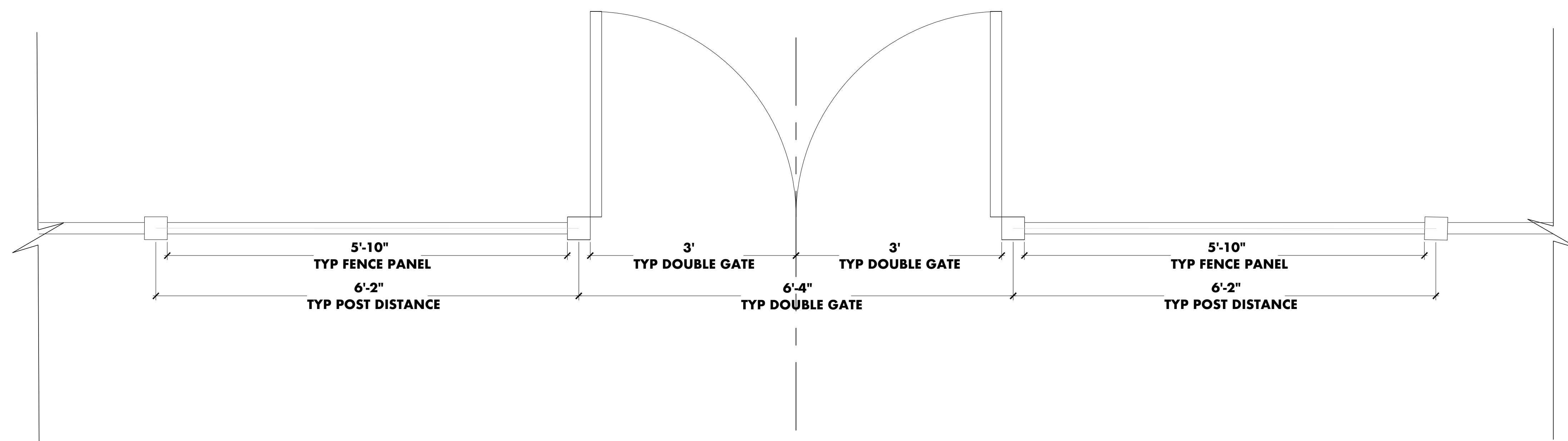
1 FENCE PLAN
