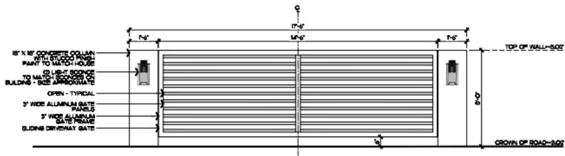
Proposed Driveway Gate Elevation Detail
