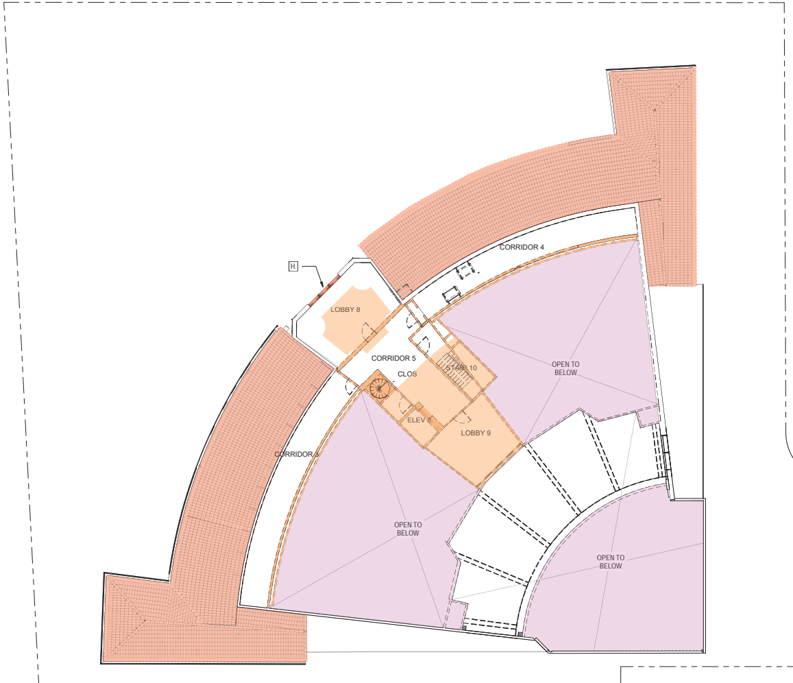
1 MATERIAL REMOVAL PLAN - LEVEL 03 - EXISTING 3/32" = 1'-0"
