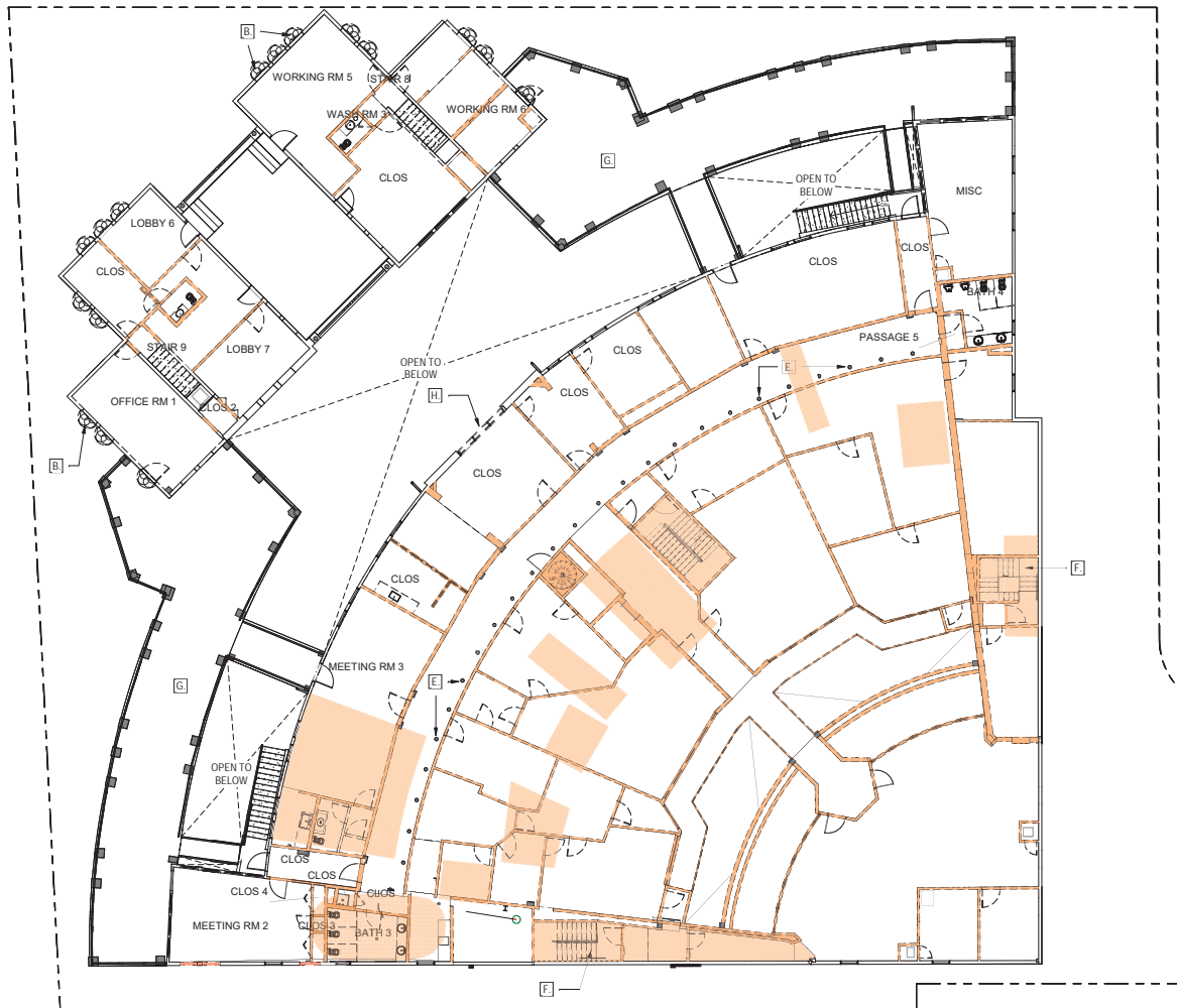
① MATERIAL REMOVAL PLAN - LEVEL 02 - EXISTING 3/32" = 1'-0"
