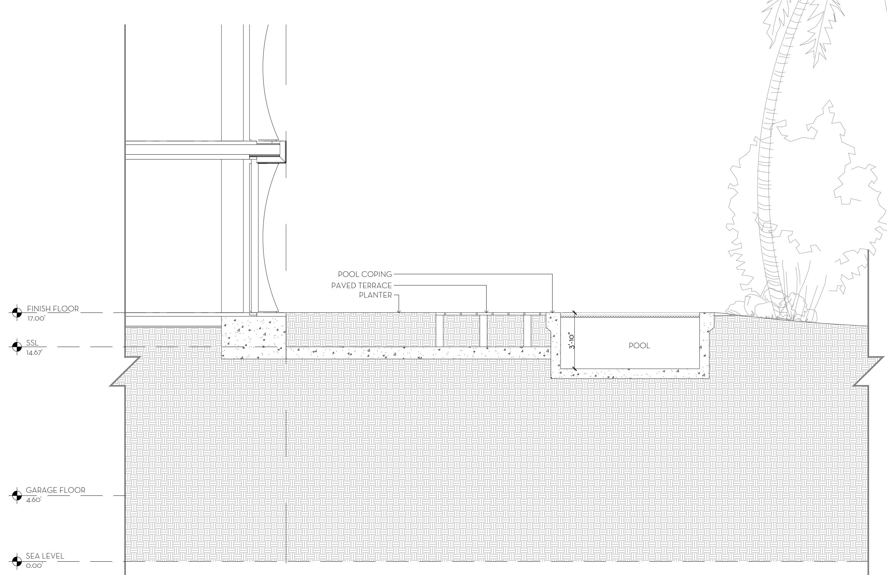
2 BUILDING 1 SOUTH POOL SECTION D2 SCALE: 1/4"=1'-0"
