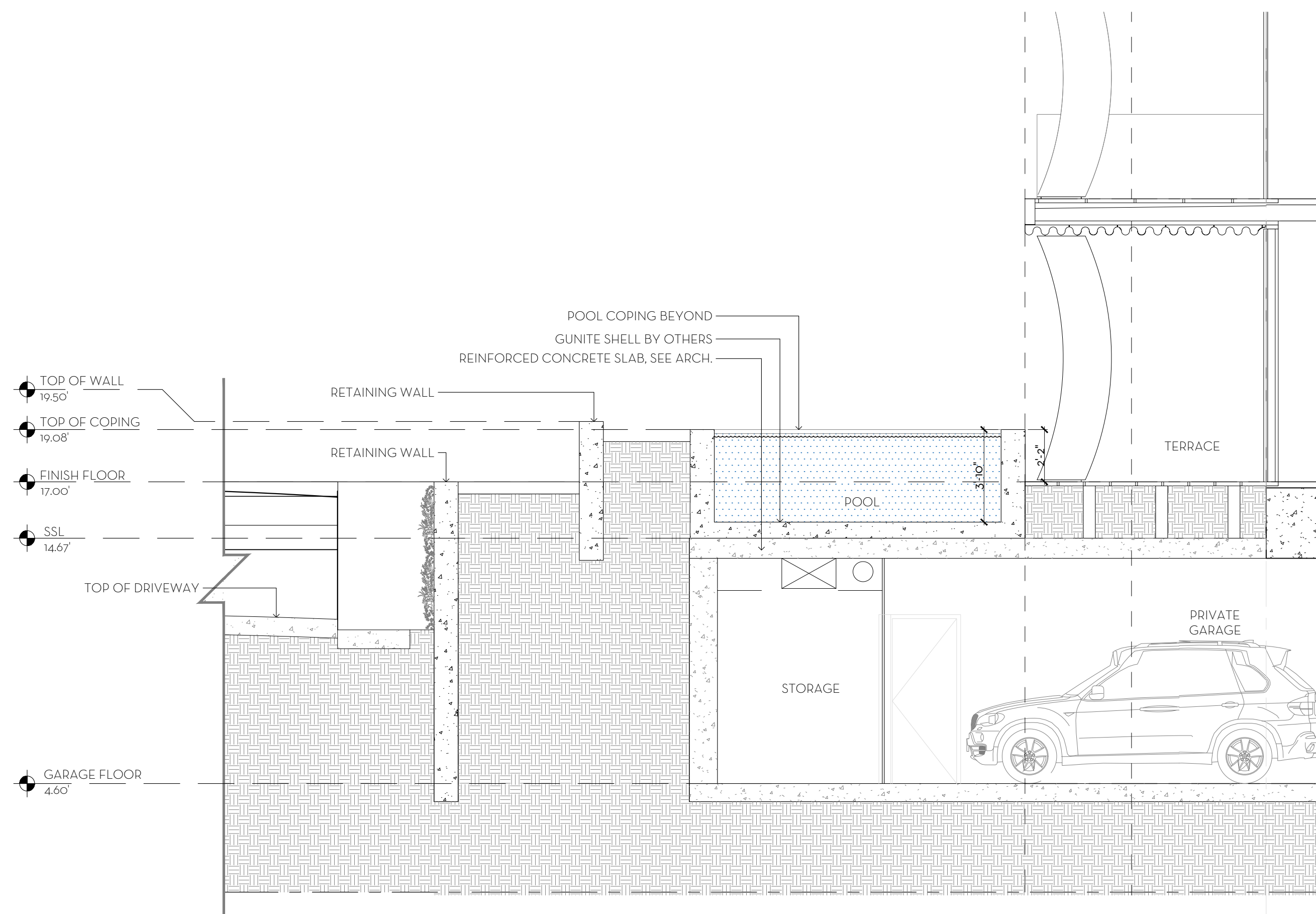
4 BUILDING 2 NORTH POOL SECTION B D2 SCALE: 1/4"=1'-0"
