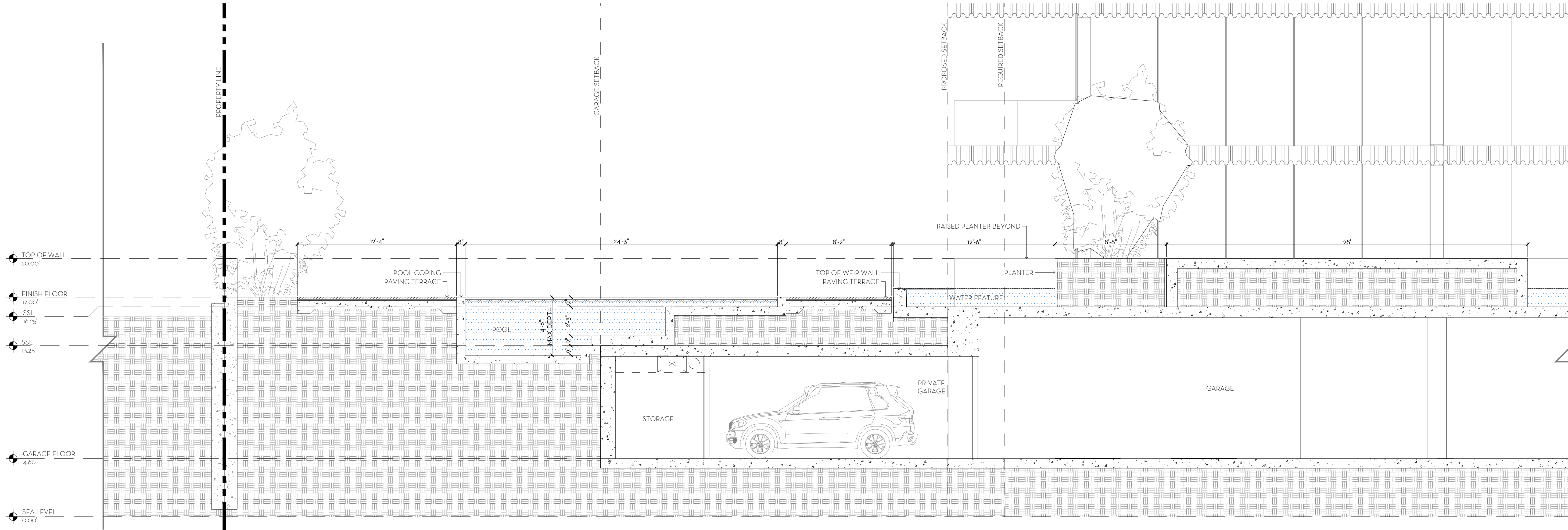
1 AMBASSADOR COURTYARD SOUTH SECTION D3 SCALE: 1/4"=1'-0"
