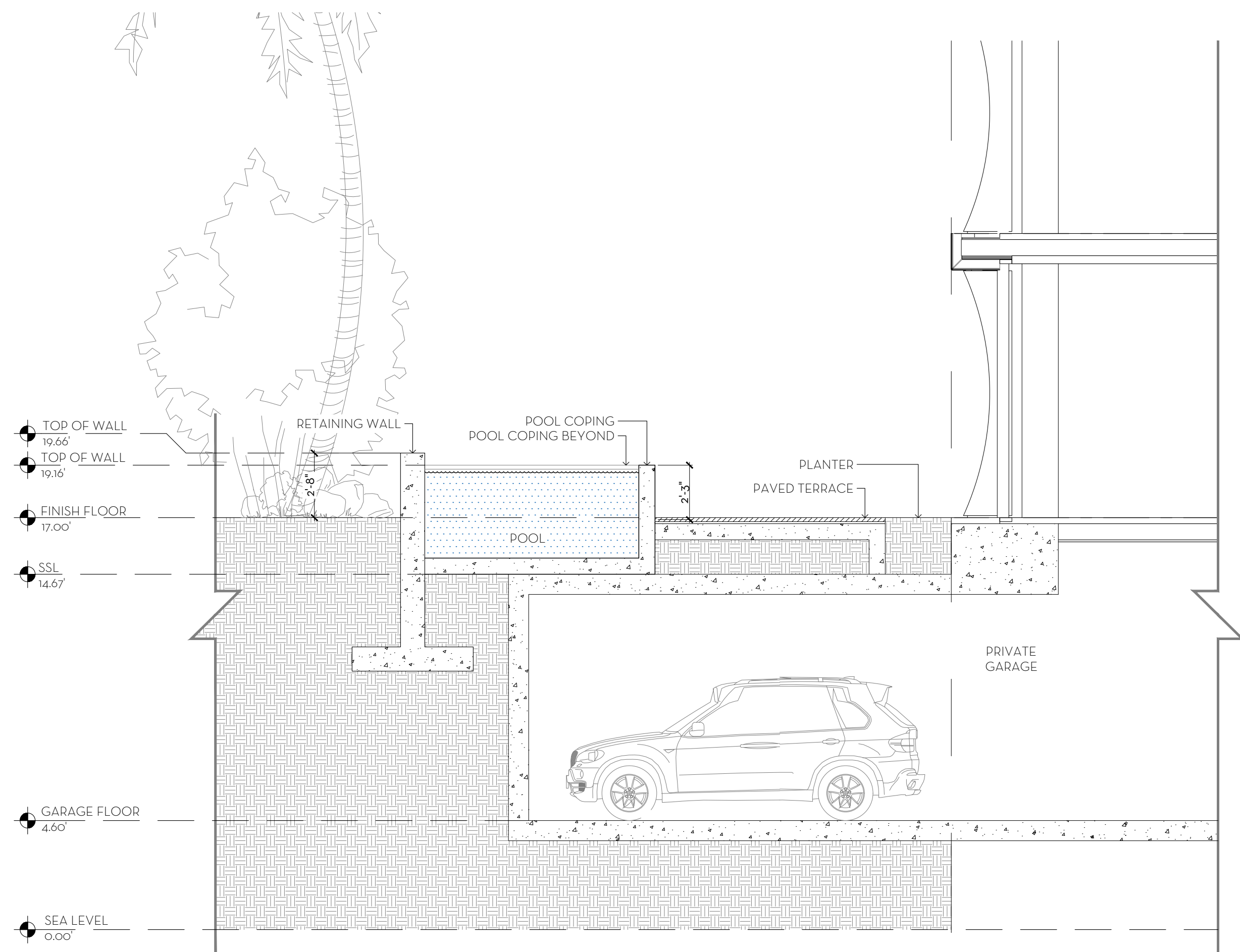
1 BUILDING 1 NORTH POOL SECTION D2 SCALE: 1/4"=1'-0"
