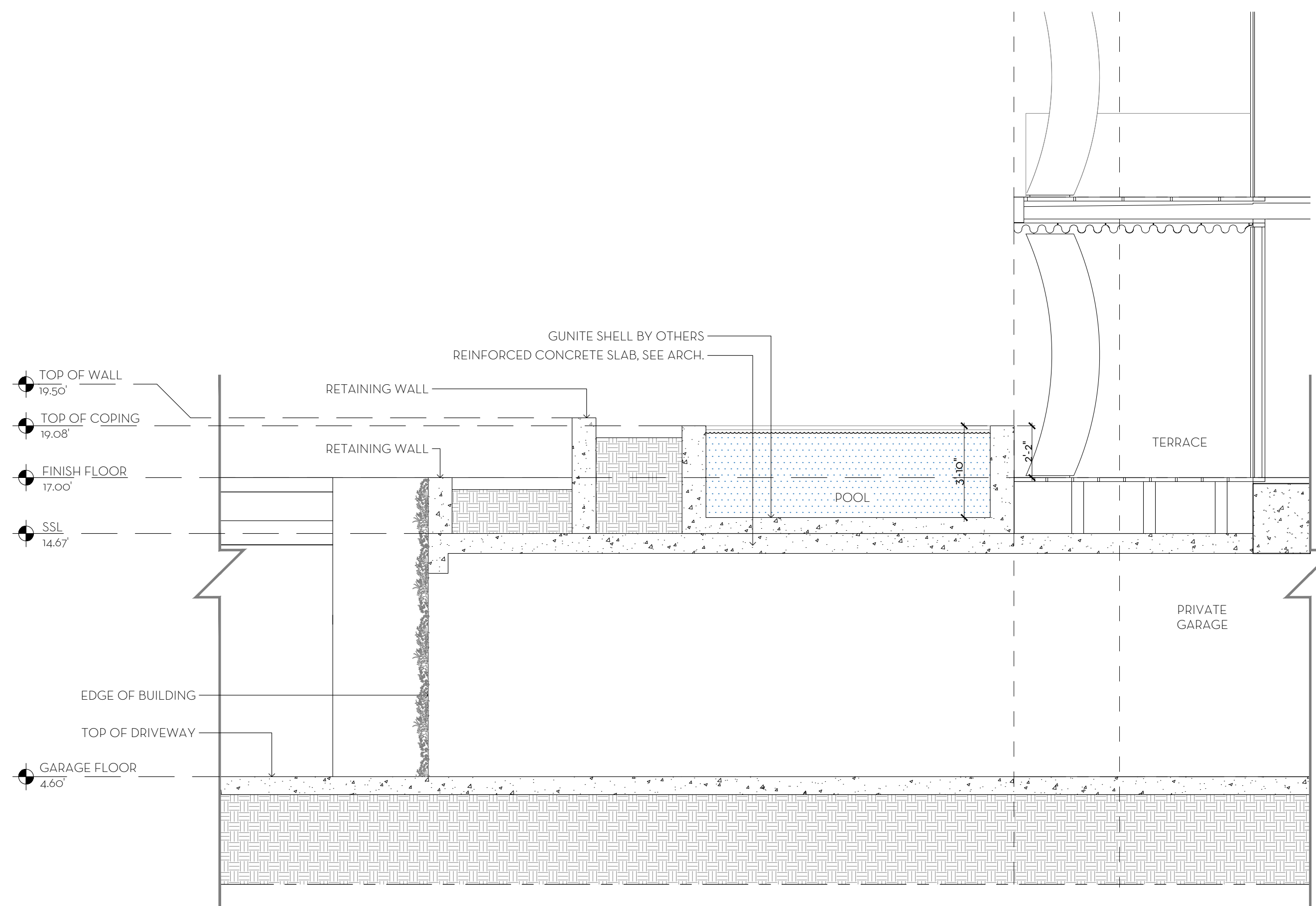
3 BUILDING 2 NORTH POOL SECTION A D2 SCALE: 1/4"=1'-0"
