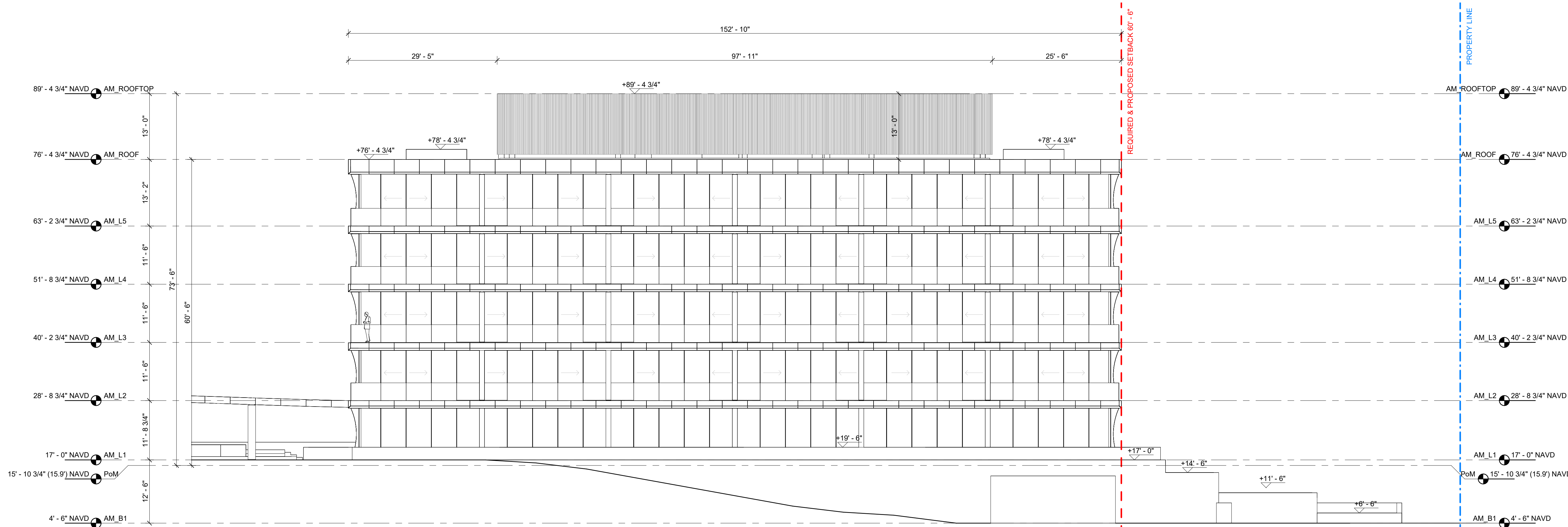
1 BUILDING 2 ELEVATION NORTH SCALE: 3/32" = 1'-0"
