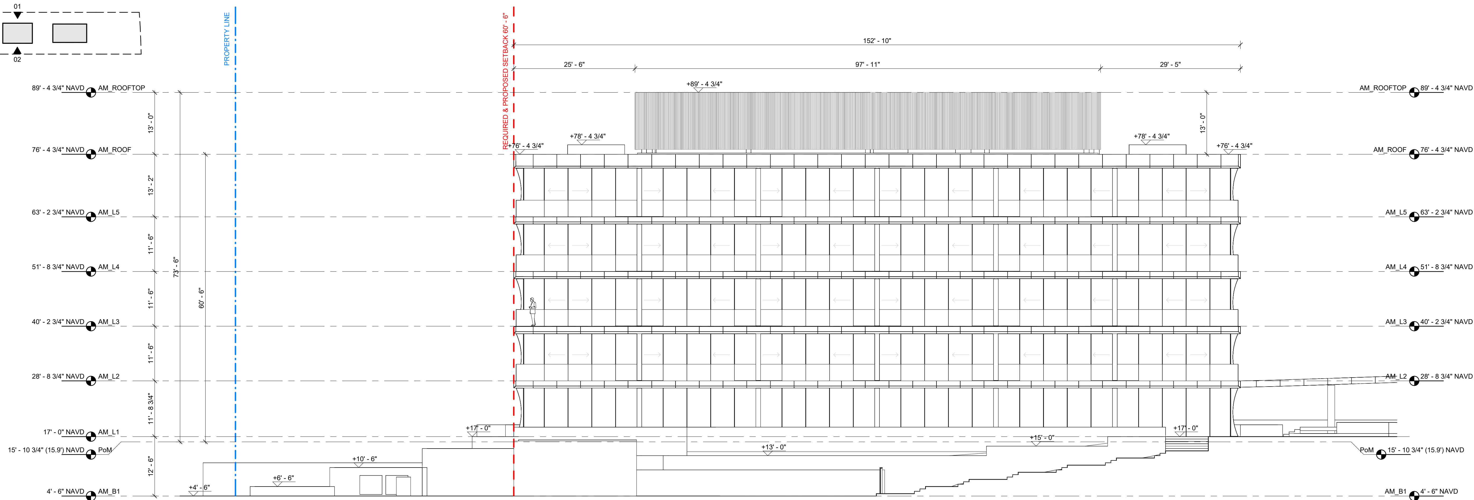
2 BUILDING 2 ELEVATION SOUTH SCALE: 3/32" = 1'-0"
