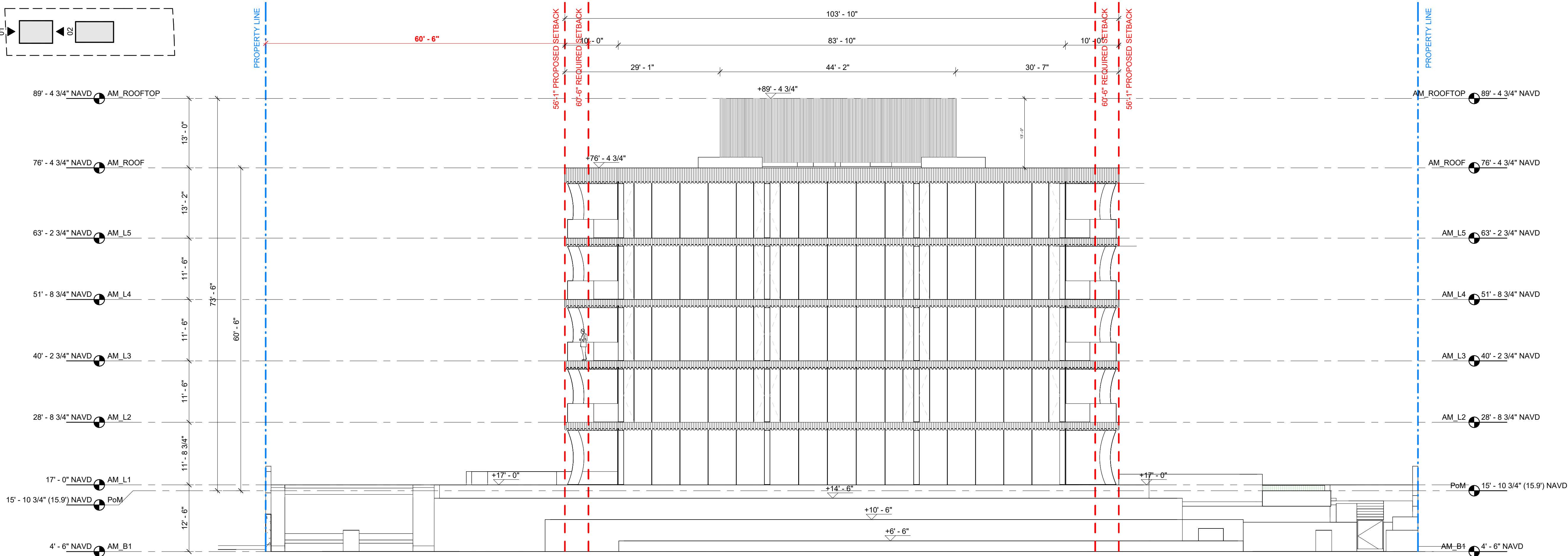
2 BUILDING 2 ELEVATION WEST SCALE: 3/32" = 1'-0"
