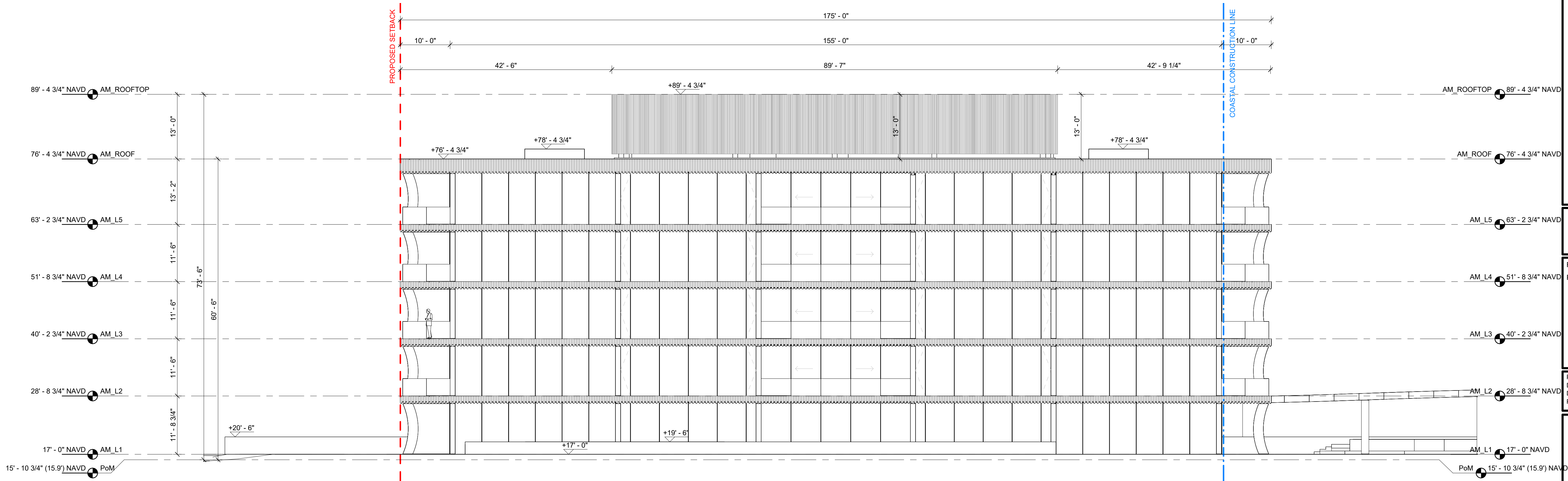
1 BUILDING 1 ELEVATION NORTH SCALE: 3/32" = 1'-0"
