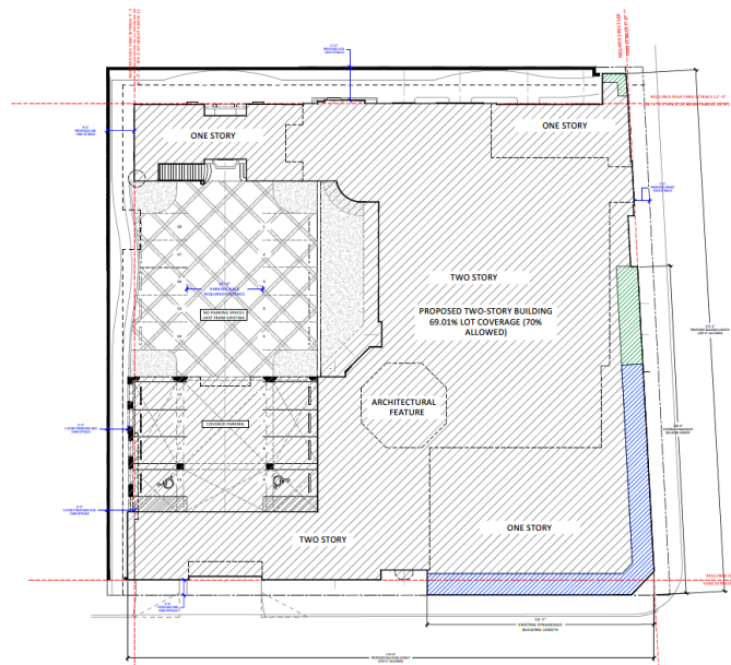
VARIANCE DIAGRAM
