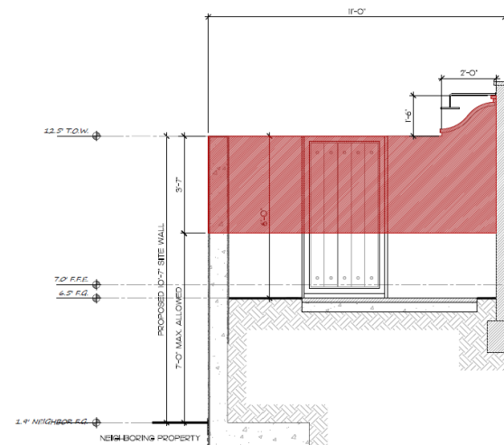
West side yard variance diagram
