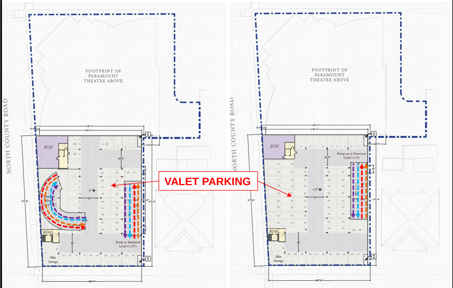
PROPOSED PLAN: BASEMENT LEVEL 2
