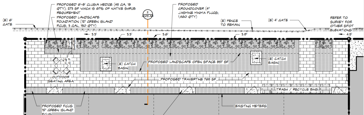
PROPOSED SITE PLAN (REAR OF PROPERTY)
